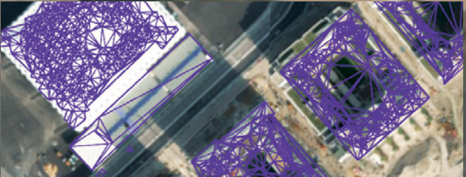
Automatic Feature Extraction (AFE) of buildings from a 0.5m, Next Generation Automatic Terrain Extraction (NGATE) DSM. Imagery courtesy of Ordnance Survey Great Britain.
